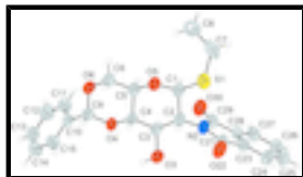
Fig. 1. Molecular structure showing 50% probability displacement ellipsoids.
