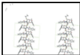
Fig. 2. Stereoview showing the intermolecular hydrogen bond intercalations between molecules forming a chain along the b-direction.
